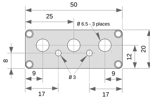
Front Faceplate
