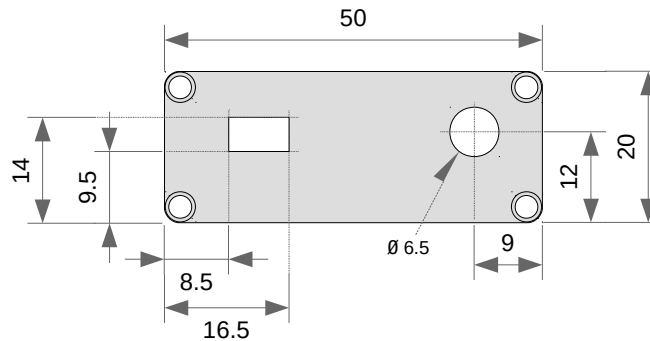
Rear Faceplate
